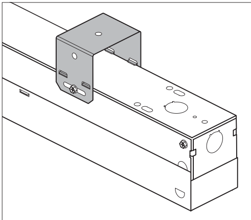
FIG C.3.2 75L Shown
